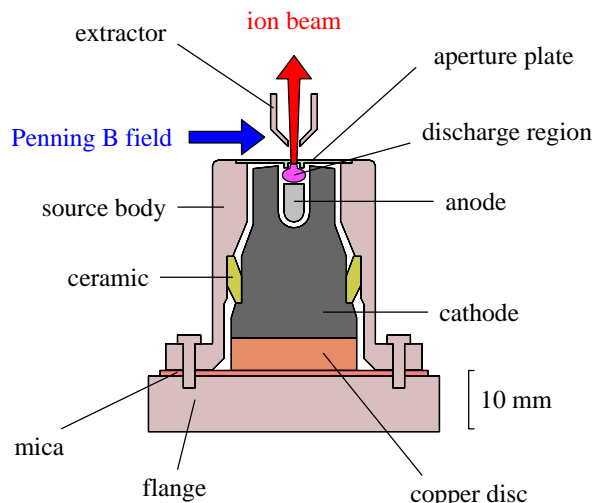
Figure 1: Schematic of the ISIS \text{H}^- ion source.
