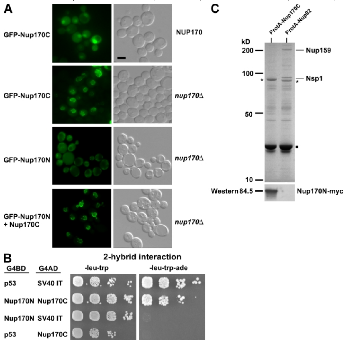
Nup170C and Nup170N physically and functionally interact with each other. (A) Nup170C tethers Nup170N to the NE. The indicated GFP-tagged Nup170 domains were expressed under the control of the NOP1 promoter in the specified strains and analyzed by fluorescence microscopy. Cells are also shown by Nomarski optics. (B) Nup170C and Nup170N show a two-hybrid interaction. The indicated constructs, fused to either the GAL4 DNA-binding domain (G4BD) or the GAL4 activation domain (G4AD), were expressed into a reporter yeast strain. Cells were spotted in 10-fold serial dilution steps onto SDC-Trp-Leu (for plating efficiency) or SDC-Trp-Leu-Ade (for two-hybrid interaction) plates and incubated at 30°C for 3 d and 4 d, respectively. (C) Affinity-purified Nup170C coenriched Nup170N. Protein A (ProtA)-tagged Nup170C and protein A-tagged Nup82 were affinity purified from a yeast strain coexpressing myc-tagged Nup170N. The TEV-eluates were analyzed by SDS-PAGE and Coomassie staining (top) and Western blotting (bottom) using anti-myc antibodies to detect Nup170N. Coenriched Nsp1 and Nup159 are indicated on the right. The asterisks label the purified bait proteins, and the dot marks the TEV protease. Bar, 5 μm.
