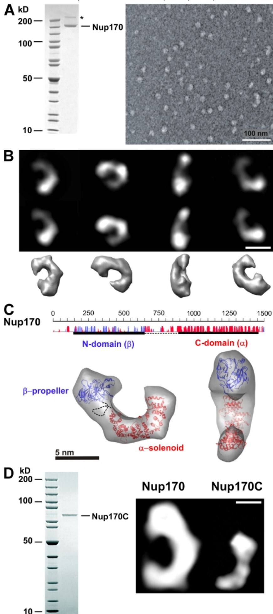
Electron microscopic single-particle analysis of purified full-length Nup170 and Nup170C. (A) Affinity-purified Nup170 was analyzed by SDS-PAGE and Coomassie staining (left; contaminated by FAS and indicated by an asterisk) and by EM (right). A charge-coupled device image overview electron micrograph of the
