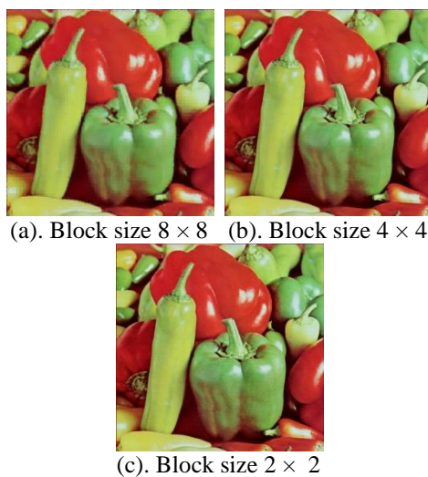
Fig.8. Pepper
