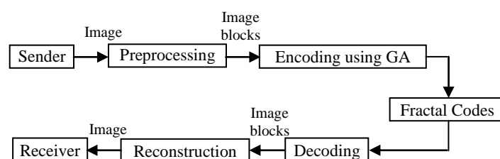
Fig.1. Architecture of the Proposed Iteration-Free Fractal Image Coding Method
