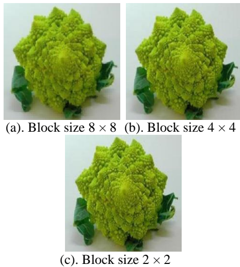
Fig.7. Cauliflower
