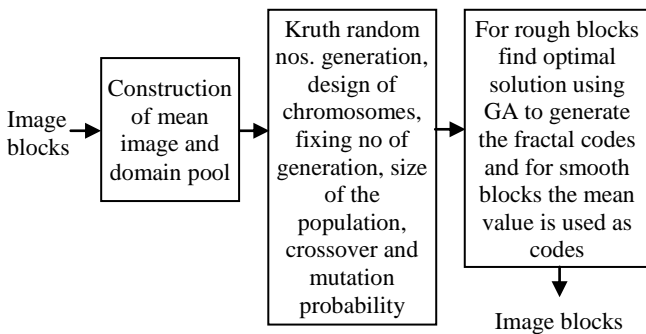
Fig.3. Proposed Encoder Using GA
