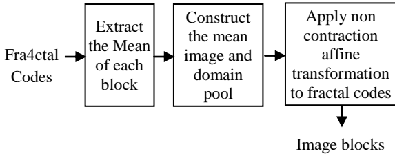
Fig.2. Proposed Decoder
