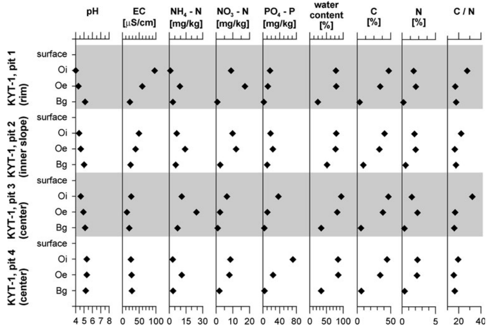
Fig. 5 Pedeochemical parameters in polygon KYT-1
